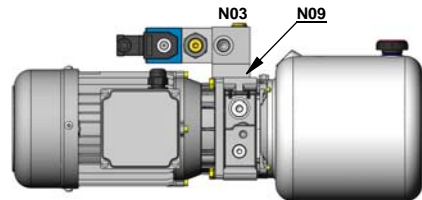
Motor IEC100 frame Coupling TR05
